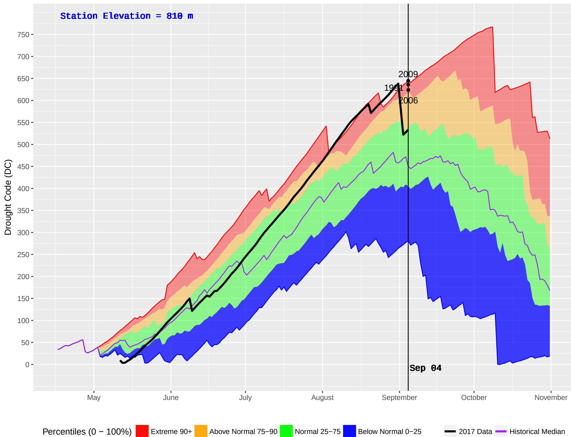
MCBRIDE LAKE (180) : Historical (1990–2016) and Current (2017) Noon Drought Code (DC)
